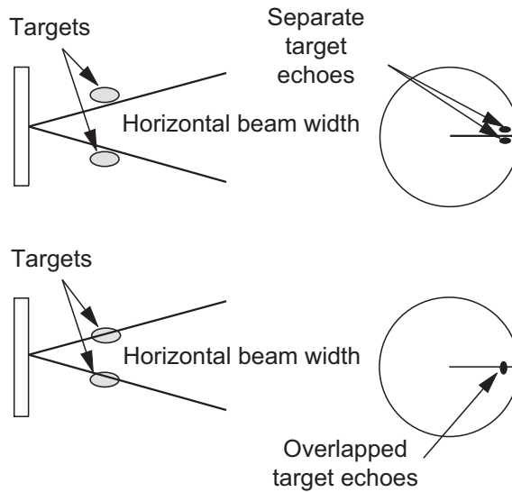
Bearing resolution
