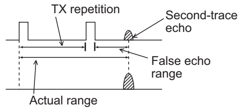
Second-trace echoes
